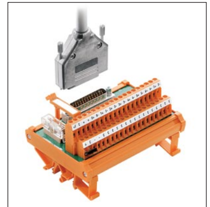
Shielded Sub-D Connector for Analog Inputs/Outputs
